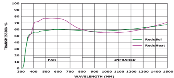
TRANSMISSION SPECTRA COMPARISON BETWEEN REDUSOL AND REDUHEAT
